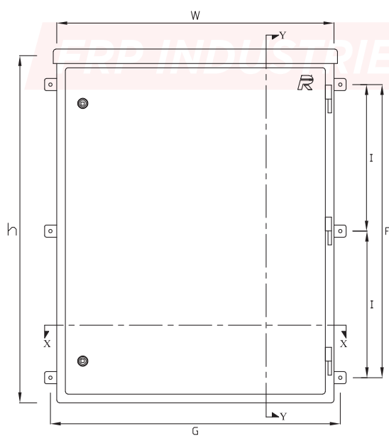
FRONT ELEVATION
