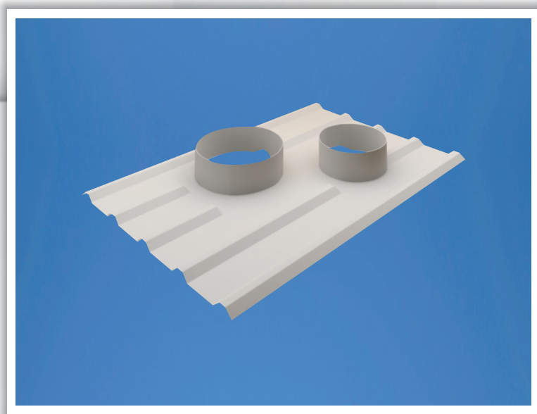
Soaker Panel with multiple openings
