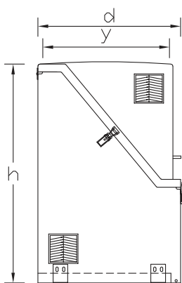
SIDE ELEVATION
