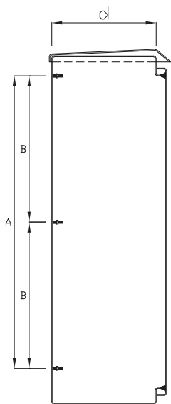
SECTION Y-Y
